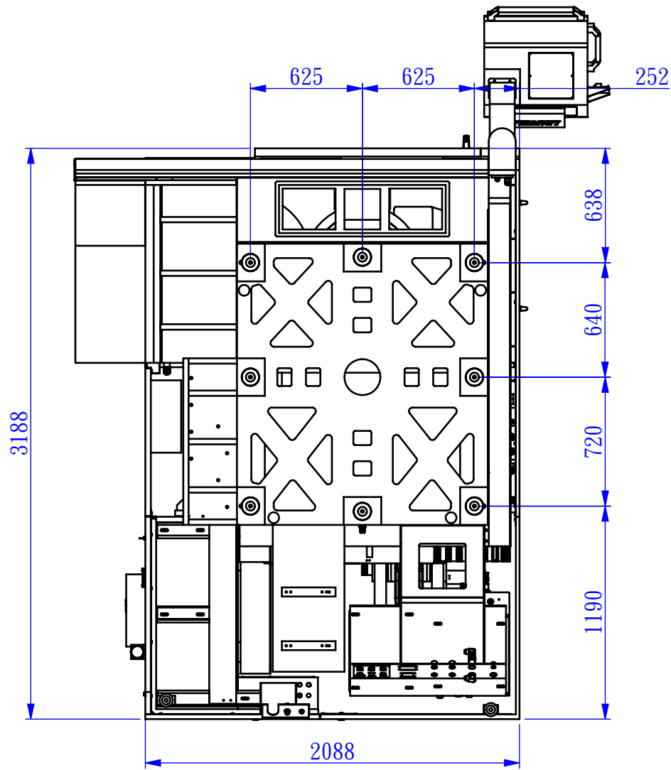
地基圖 FOUNDATION DRAWING NO:UW02000500
