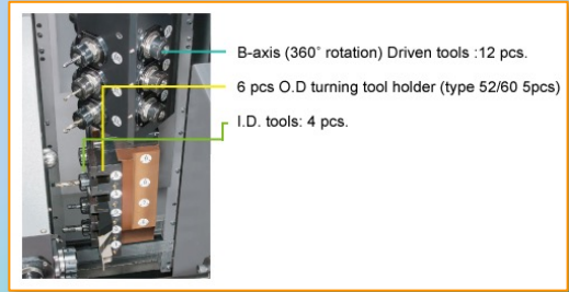
tooling system for the main spindle (sharing 360° B-axis with sub-spindle operation)
