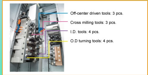
tooling system for the sub-spindle
